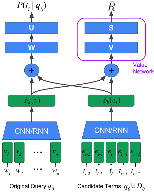
Figure 2: An illustration of our neural network-based reformulator.
